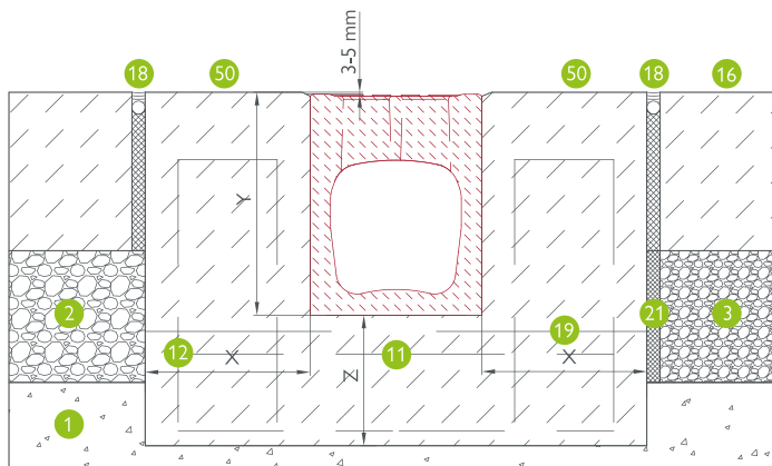
BG-FILCOTEN® one, NW 150: Concrete – Concrete, class D – F
