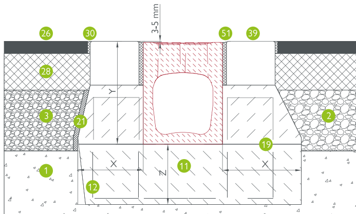
BG-FILCOTEN® one, NW 150: Asphalt – Asphalt, class D – F
